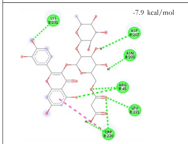
Figure 1: Molecular Docking of 3RUK_Quercetin
