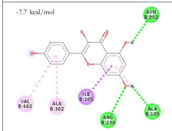
Figure 2: Molecular Docking of 3RUK_Kaempferol
