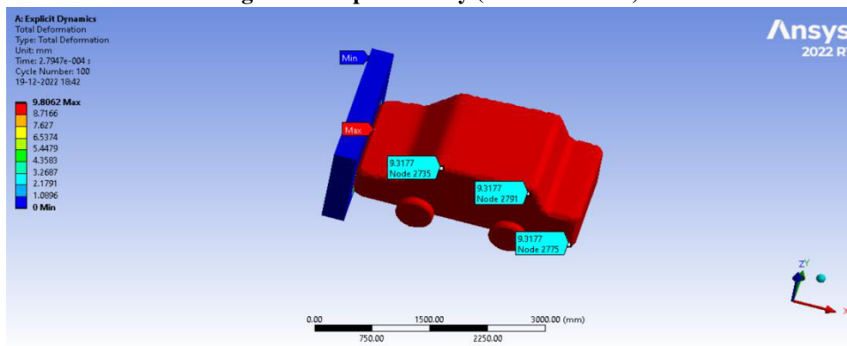
Figure 15: Total deformation
