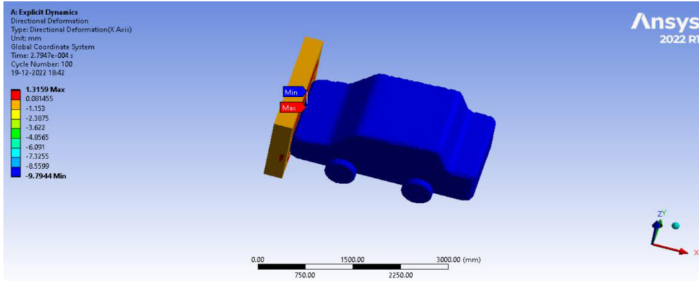
Figure 16: Directional deformation
