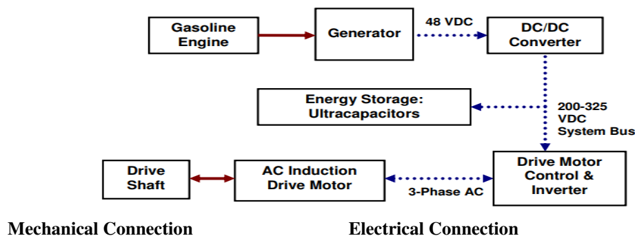
Figure 1: Block Diagram of our Series Hybrid System
