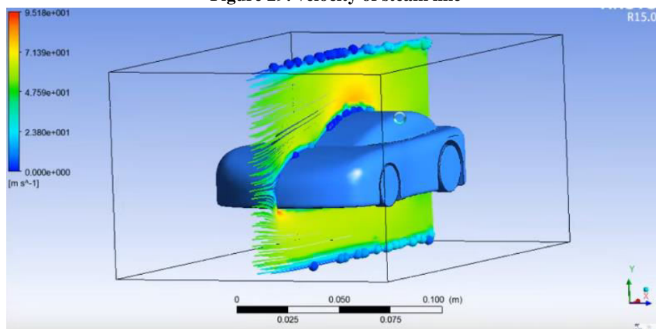
Figure 30: racing car velocity of steam line
