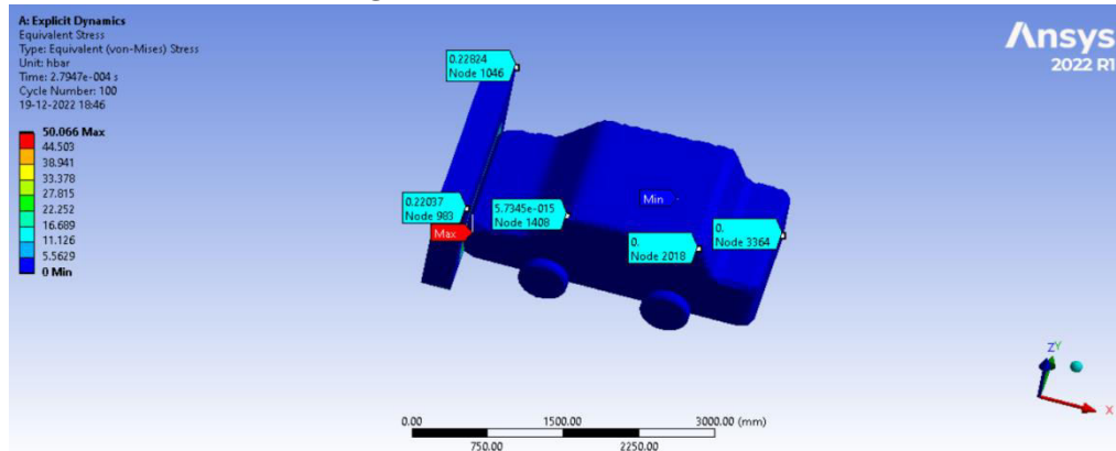
Figure 17: Equivalent stress
