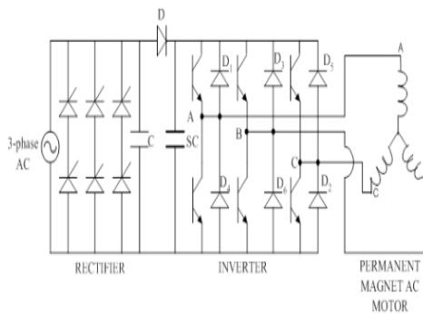
Fig. 4. PMAC motor fed from a voltage source inverter.
