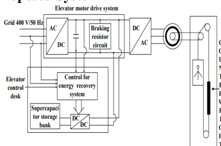
Fig. 1. System configuration.
