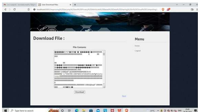
Fig 4.3 Decrypted Data
