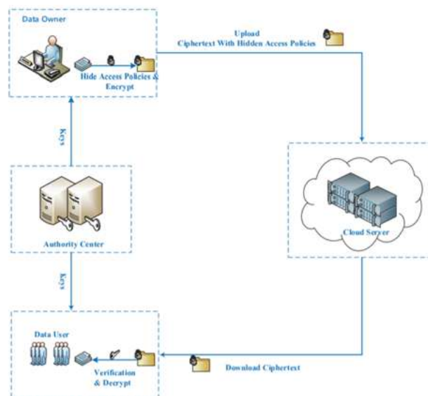
Fig 1: System Model
