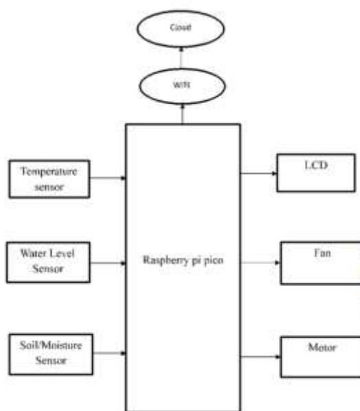
Fig:1. Block Diagram of Smart Farming WIFI Based Agriculture System
