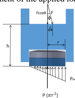
Fig. 7.1 valve leakage analysis
