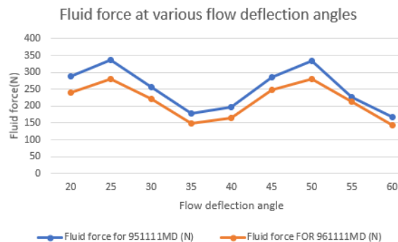
Fig. 6.2 Fluid force at various deflection angles
