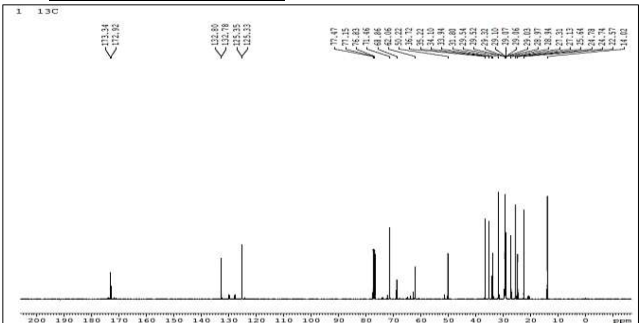
Fig.11. C 13 NMR of castor oil-based polyol.
