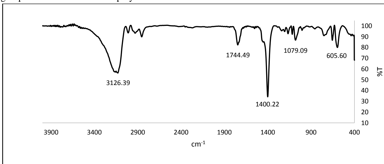
Fig.13. FT-IR Spectra of the polyol.
