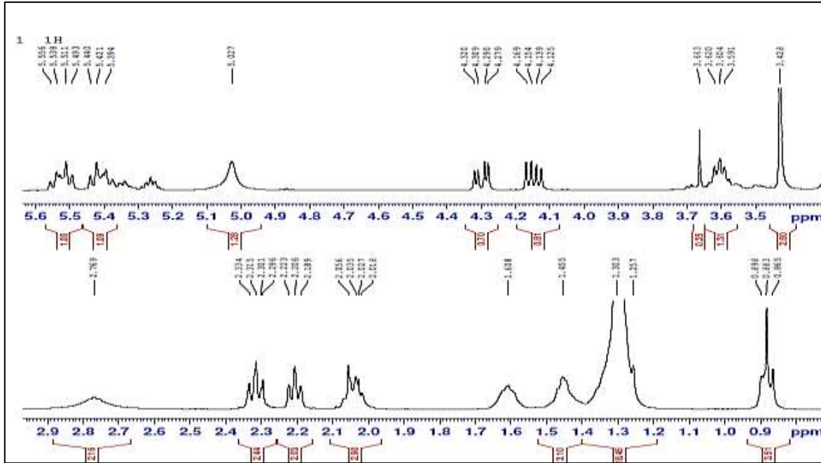
Fig.10. H 1 NMR of castor oil-based polyol
