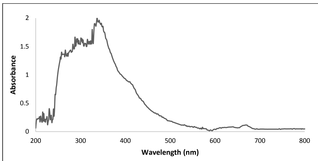
Fig.12. UV absorption spectra of the castor oil polyol.
