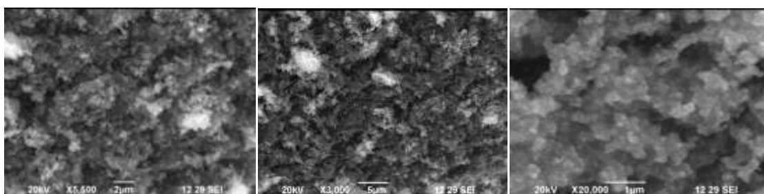
Fig. 6. SEM images of the Nano-silica obtained from the bamboo leaves ash
