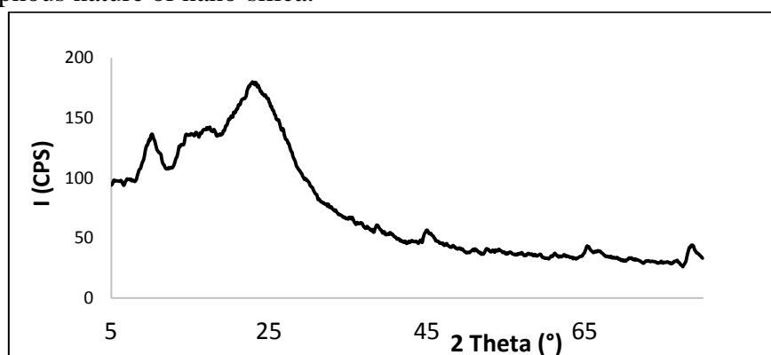
Fig. 5. X-Ray Diffraction pattern of Nano-silica.
