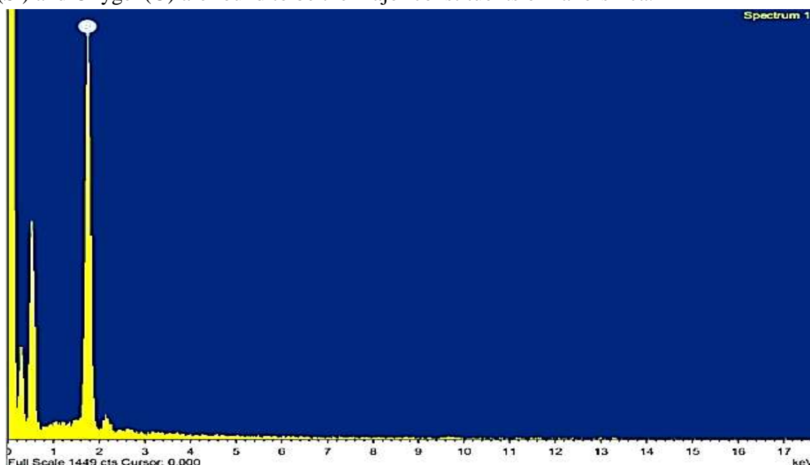
Fig.7. Energy Dispersive X-Ray spectrum of Nano-silica
