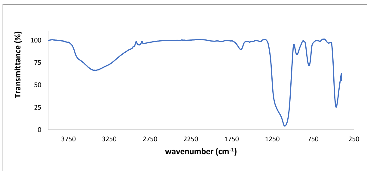
Fig. 4. Fourier Transform- Infra Red spectral analysis of the prepared Nano-silica.
