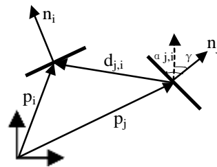
Figure 2 Local convexity
