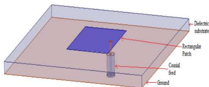
Figure [3] Co-axial probe fed rectangular patch antenna (10GHz)
