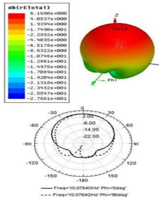
Figure [5] a), Radiation pattern of co-axial fed rectangular patch antenna at operating frequency of 10.0754GHz for \phi=0^\circ & 90^\circ and b) 3D radiation energy
