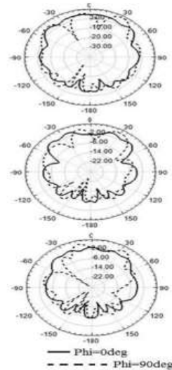
Figure [8] Radiation pattern of co-axial fed rectangular patch antenna a) LP=0.2cm, PS=0.6cm operating at 31.3618GHz, b) LP=0.2cm, PS=0.55cm operating at 33.1759GHz & c) LP=0.2cm, PS=0.5cm operating at 34.8643GHz
