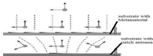
Figure [1] Radiation principle of patch antenna tuned with Met material structure
