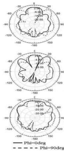
Figure [10] Radiation pattern of co-axial fed rectangular patch antenna a) LP=0.3cm, PS=0.6cm operating at 28.5327GHz, b) LP=0.3cm, PS=0.55cm operating at 29.799GHz & c) LP=0.3cm, PS=0.5cm operating at 30.9296GHz
