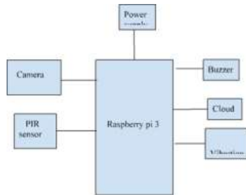
Figure 1. Block diagram of advanced security system
