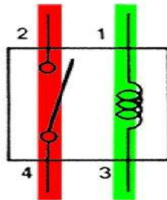
relay operation
