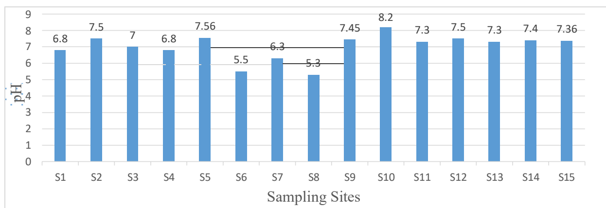
Figure 1: Variation of pH in sampling sites ground water of Kishangarh block
