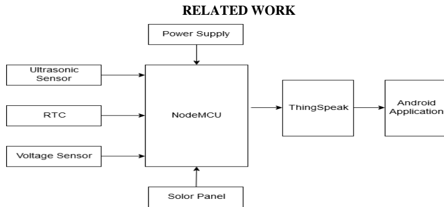
Fig 4.1 Architecture of smart dustbin
