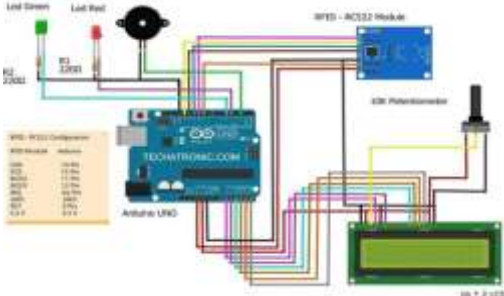
Fig 6 circuit diagram
