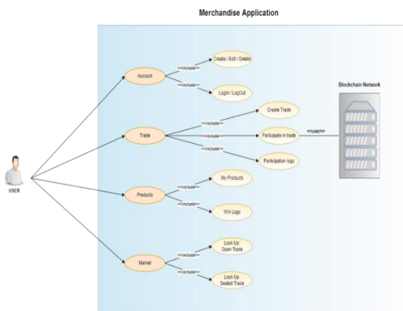
Fig. 3. Use Case Diagram of the proposed system
