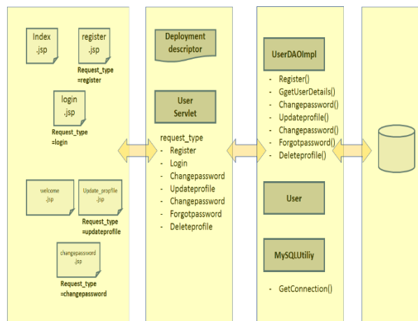
Fig. 1. Data flow diagram of the proposed system
