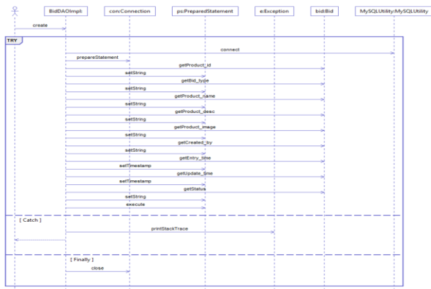
Fig. 4. Initial Sequence Diagram
