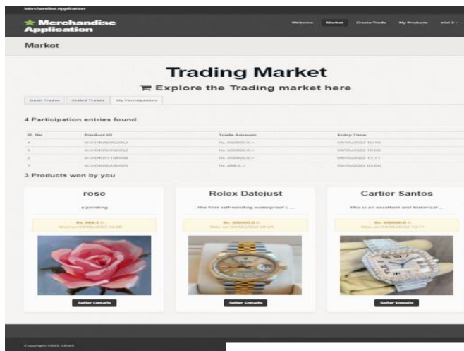
Fig. 12. Market Page
