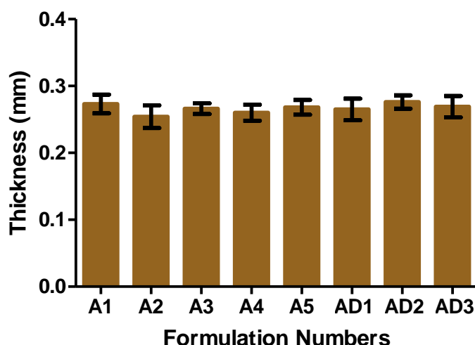
Figure No. 2: Measurement of Thickness of transdermal patches of different formulations
