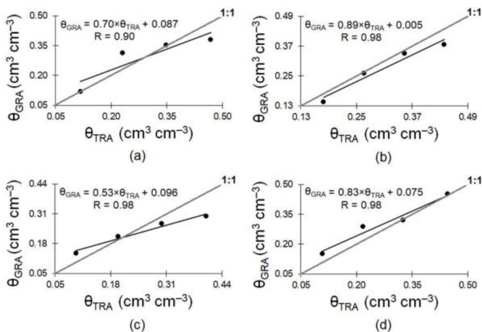
Figure 6. Comparison of the soil water content ( \theta ) evaluated by the traditional ( \theta_{\text{TRA}} —Equation (4)) and simplified gamma-ray attenuation ( \theta_{\text{GRA}} —Equation (11)) methods (1:1 line) for the contrasting soils: (a) Heavy Clay (HeCa), (b) Clay (Cl), (c) Sandy Clay Loam (SaCLo), and (d) Silt Loam (SiLo). The error bars for \theta_{\text{GRA}} are not presented in the graphs due to their magnitudes (varied from 0.0002 to 0.0016 \text{cm}^3 \text{cm}^{-3} ). \theta_{\text{TRA}} was kept constant during the experimental procedure.
