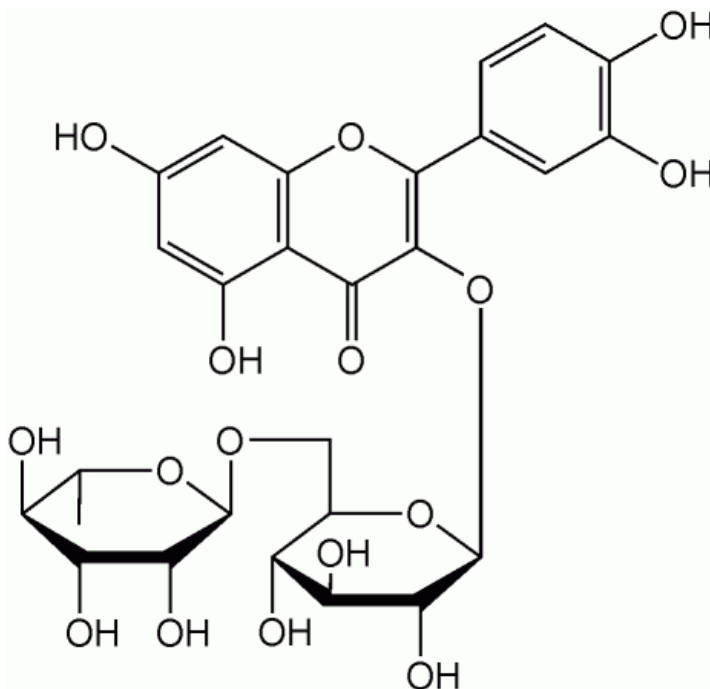
Structure of Rutin
