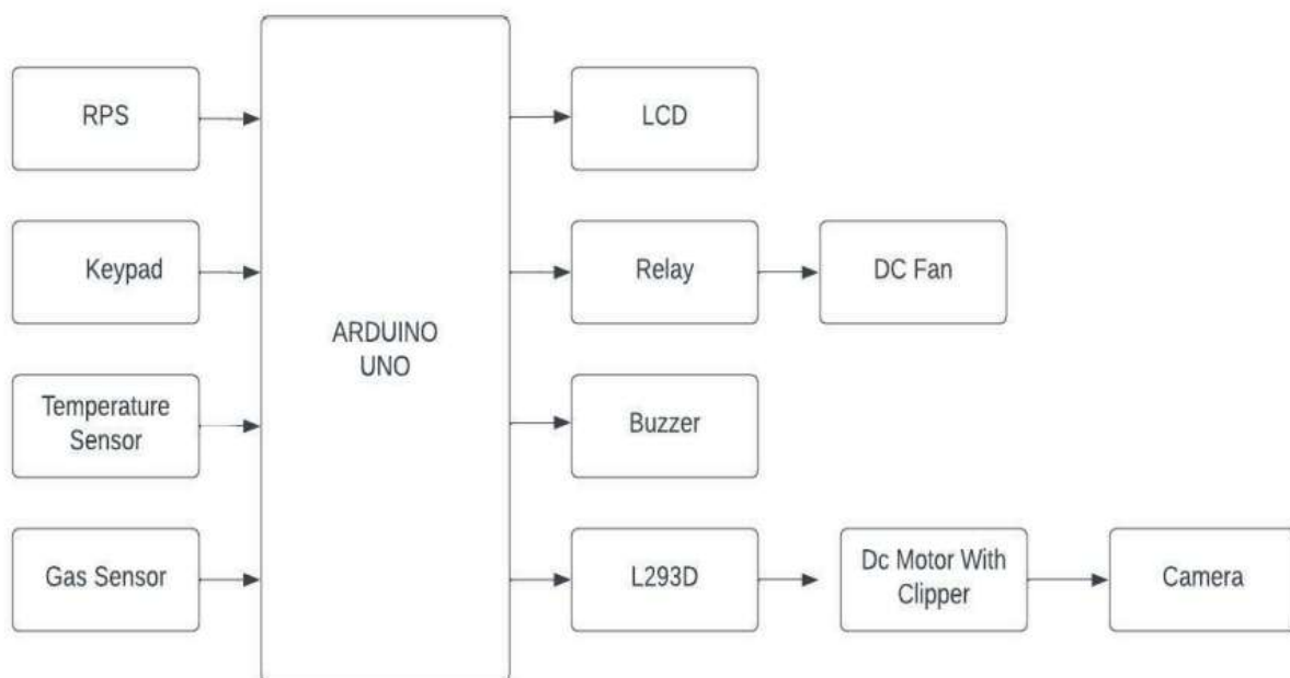
Fig 2 Block diagram
