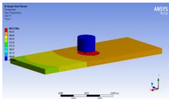
Total temperature for truncated tool
