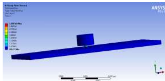
Total heat flux for tapered tool
