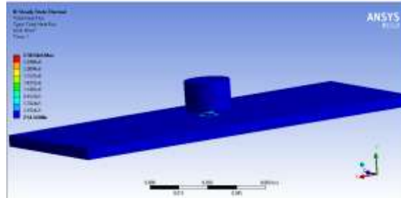
Total heat flux for pentagon tool
