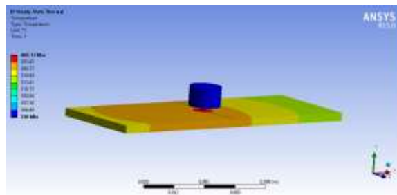
Total temperature for tapered tool
