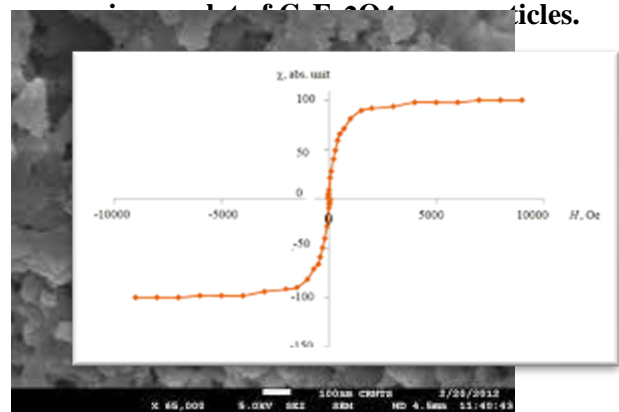
Fig. 3: Hysteresis loop for CrFe 2 O 4 nanoparticles
