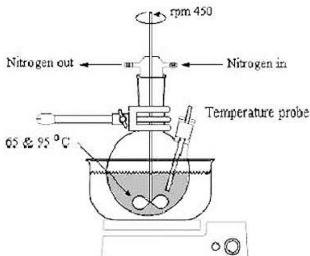
Fig. 2: Reaction vessel for microsphere preparation by liquid-liquid suspension polymerization 10 .
