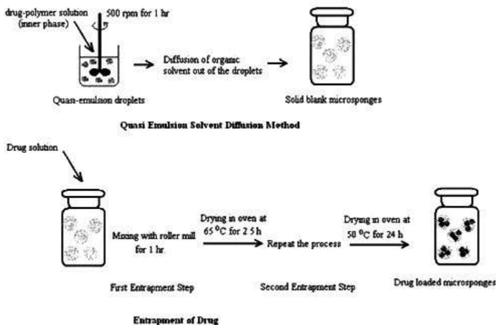
Fig. 3: Method of quasi-emulsion solvent diffusion 13 .
