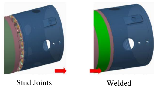
Figure 5 Simplified DFA Welded Actuator Housing
