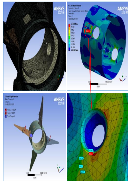
Figure 12 FEA model & Von Mises Stress of Case - II
