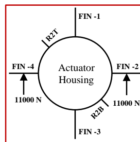
Figure 8 Pitch Loading Configuration (Case-II)
