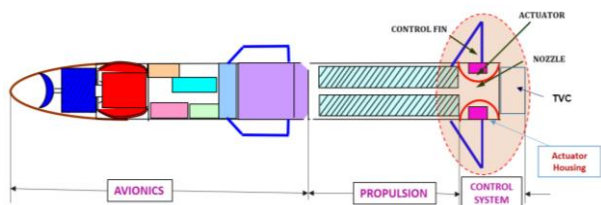
Figure 1 General Missile Configuration
