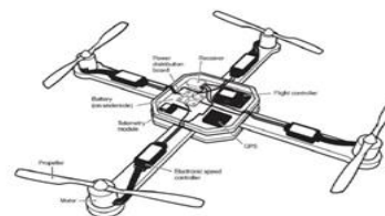
Figure : 6 Overall structure of the Drone
