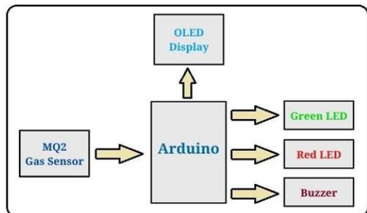
Figure 1. Block Diagram of Measuring CO2 Concentration In Air
