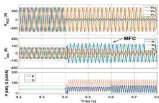
Figure 2. MFC process
