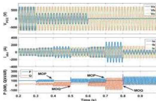
Figure 1.MOP & MOQ process
