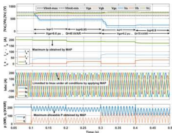
Figure 3. MAP process
