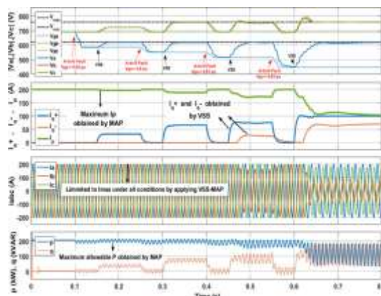
Figure 4.VSS-MAP method
