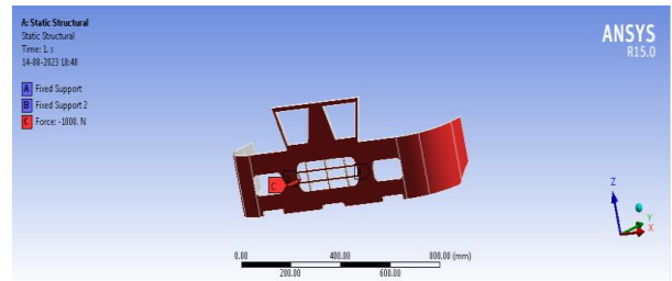
Figure 47 Boundary conditions Force: 1000N on car bumper
