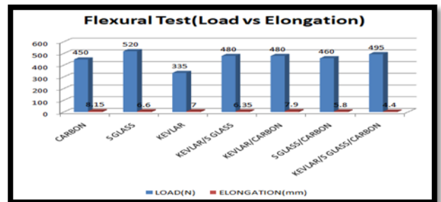
Graph 2 Flexural test result graph
