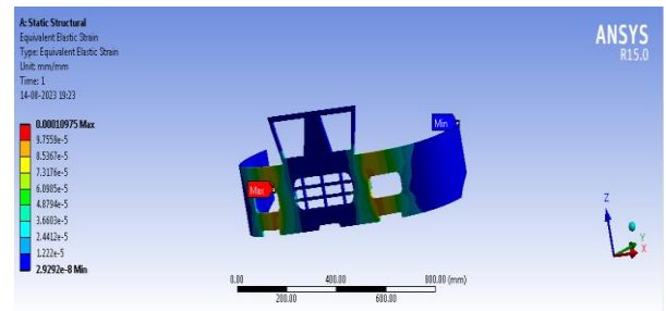
Figure 55 Strain of KSC Material
