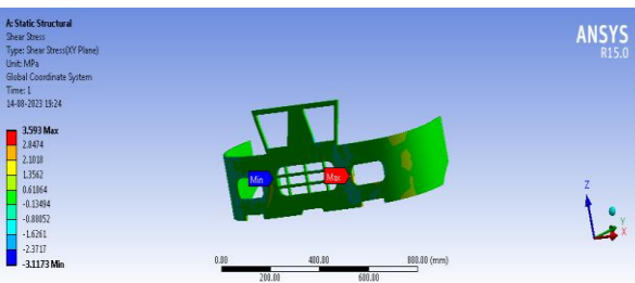
Figure 54 Shear stress of KSC Material
