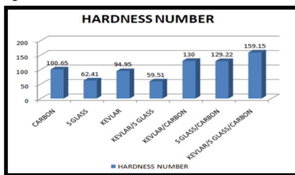
Graph 4 Hardness number result graph
