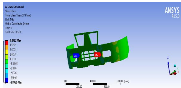
Figure 51 Shear stress of Polypropylene material
