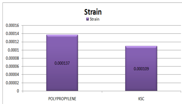
Strain graph
