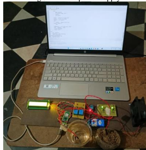
Fig 6. With power supply
