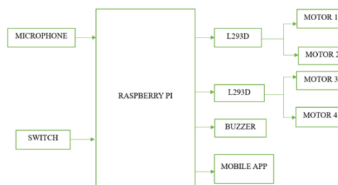
Figure 2: Block Diagram
