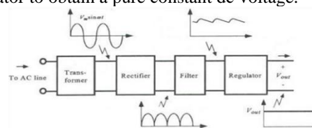
Figure 5: Block Diagram of Power Supply
