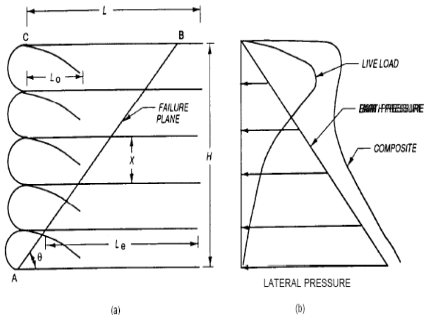
Figure 1. General Configuration of a Geotextile Retained Soil Wall and Typical Pressure Diagrams
