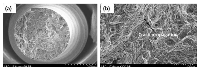
Fig 7. SEM fractography micrographs of 60 \mu\text{m} horizontal built
