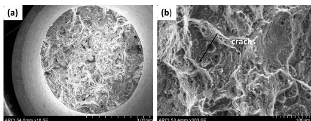
Fig 9. SEM fractography micrographs of 60µm vertical built
