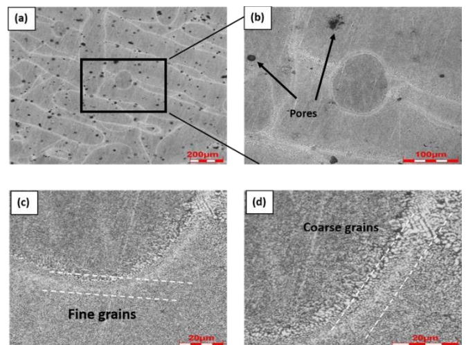
Figure 4. Optical images of AlSi10Mg @ 60 \mu m layer thickness (a) microstructure @ 200X (b) Microstructure @ 693X magnification and (c) Microstructure @ 2000X (d) microstructure @ 4000X
