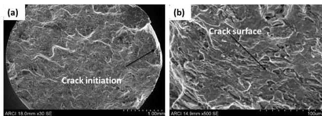
Fig 8. SEM fractography micrographs of 30µm horizontal built
