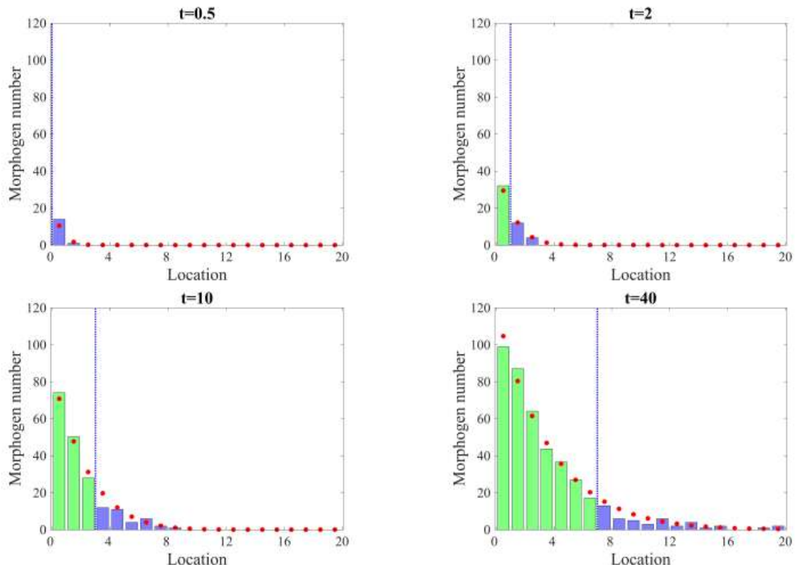
Fig. 6 Comparison between one realization of the number of morphogens using Scheme 1 with a moving interface, given in Table 3 (green bars and blue bars for the morphogen numbers in
