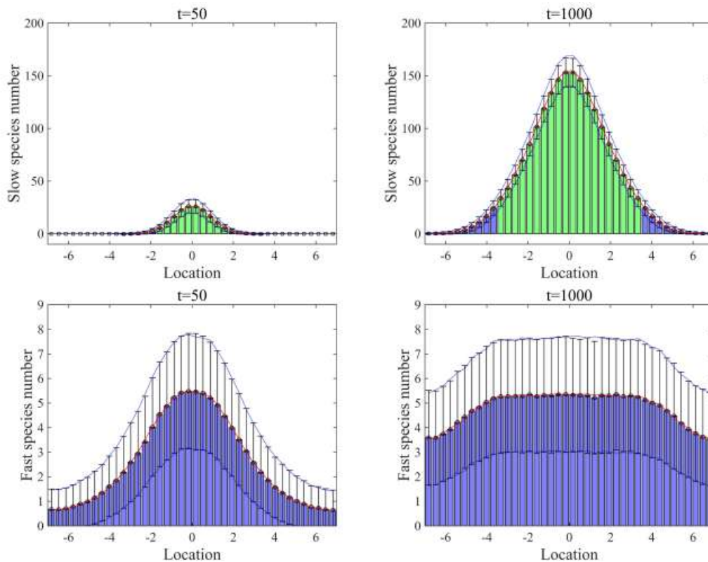
Fig. 8 Mean numbers of the molecules of slow-diffusing pomlp clusters and fast-diffusing pomlp particles, and their standard deviations from the means at t = 50, 1000 s computed
