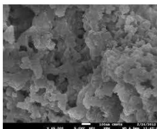
Fig.2: SEM image of CrFe 2 O 4 nanoparticles
