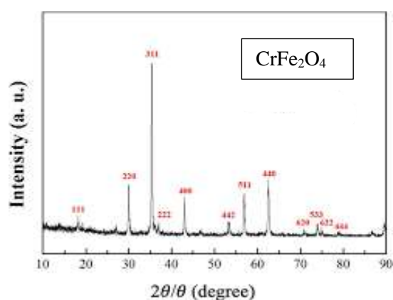
Fig.1: X-ray diffraction (XRD) pattern of CrFe 2 O 4 nanoparticles.
