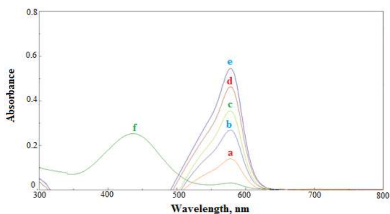
Fig.5. Final spectrum of 100 µg FSD for the 1 st method measured against Blank(B), Distilled water(A) and Blank measured against distilled water (C)
