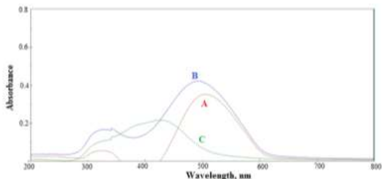
Fig.7. Final spectrum of 100 \mu\text{g} FSD for the 3rd method measured at Blank(A), Distilled water(B) and Blank measured against distilled water (C)
