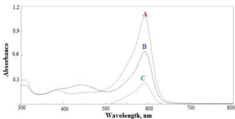
Fig.5. Final spectrum of 100 µg FSD for the 1 st method measured against Blank(B), Distilled water(A) and Blank measured against distilled water (C)
