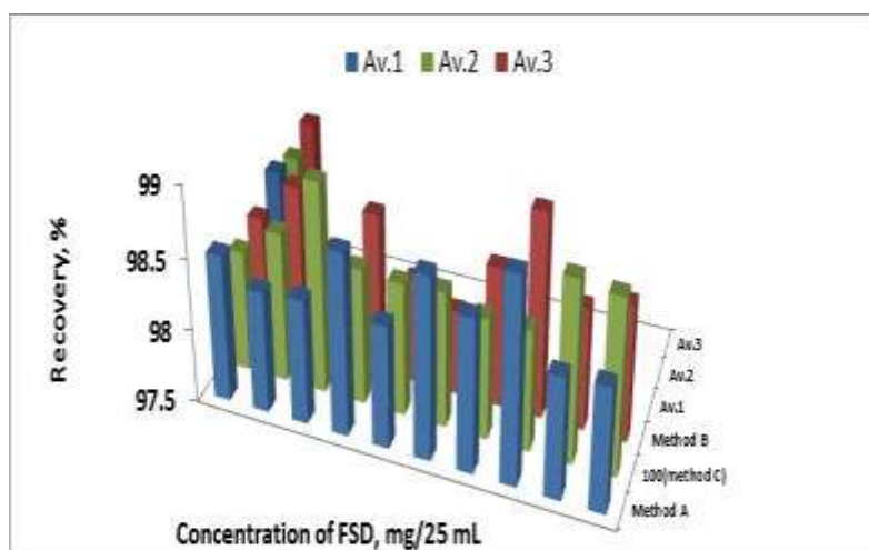
Fig.8. Accuracy and precision
