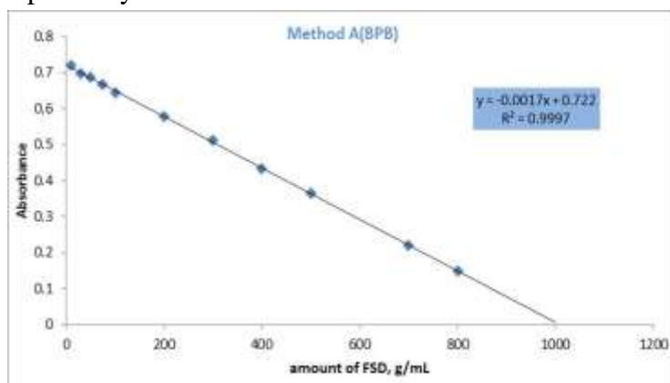
Fig.2. Calibration curve for the first method
