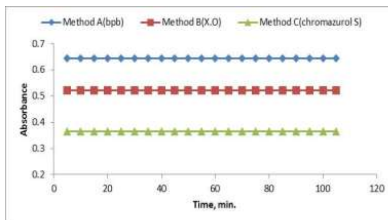
Fig. 1. Stability of the product coloured complex
