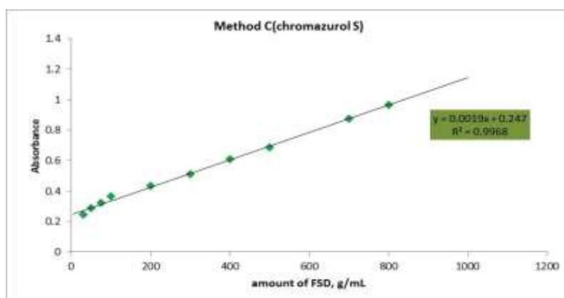
Fig.4. Calibration curve for the third method
