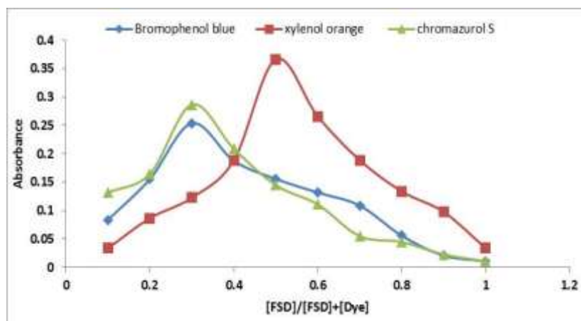
Fig 9. Job's plot of the proposed methods.
