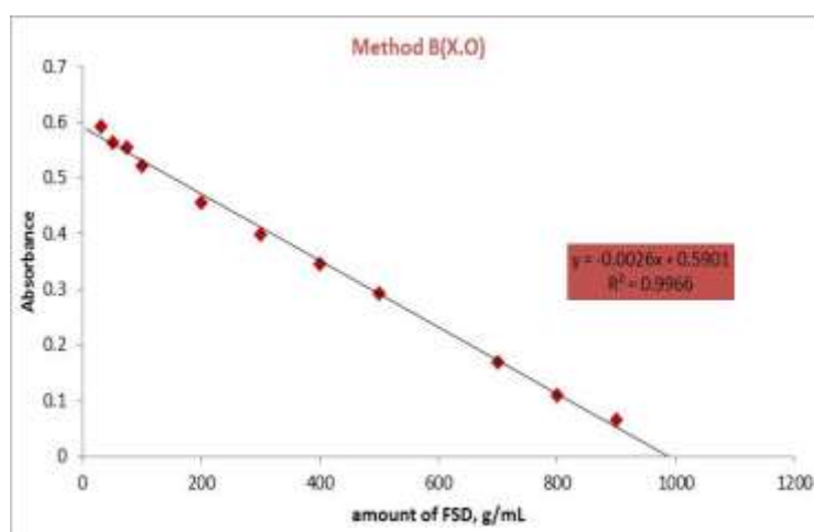
Fig.3. Calibration curve for the second method
