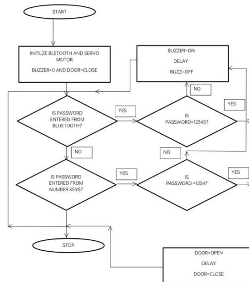
Fig:2.Block Diagram
