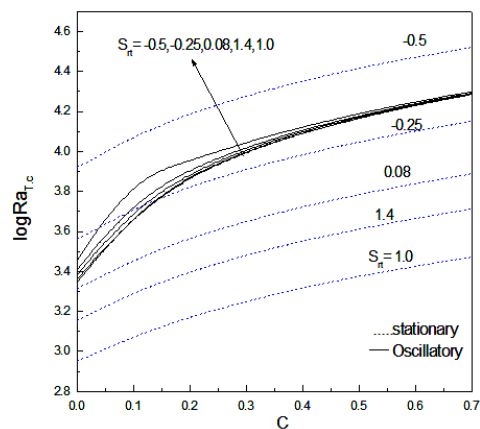
Fig. 13. Neutral stability curves for different values of S_n
