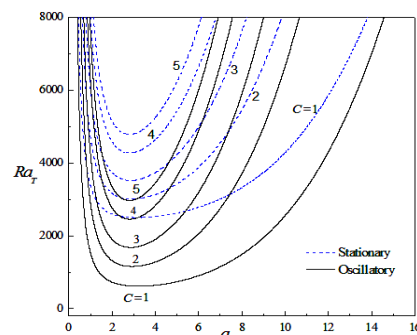
Fig. 2. Neutral stability curves for different values of C .
