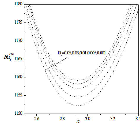
Fig. 11. Oscillatory neutral stability curves for different values of D_{fr} .
