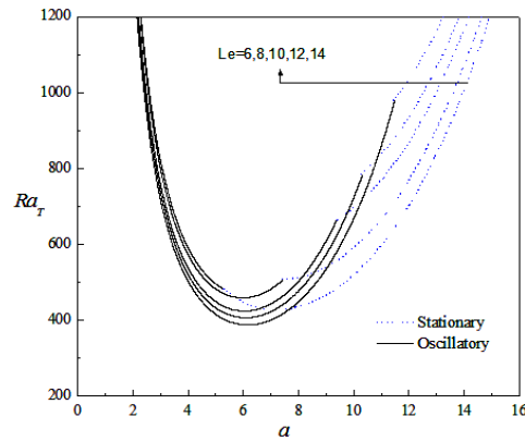
Fig. 6. Neutral stability curves for different values of Le
