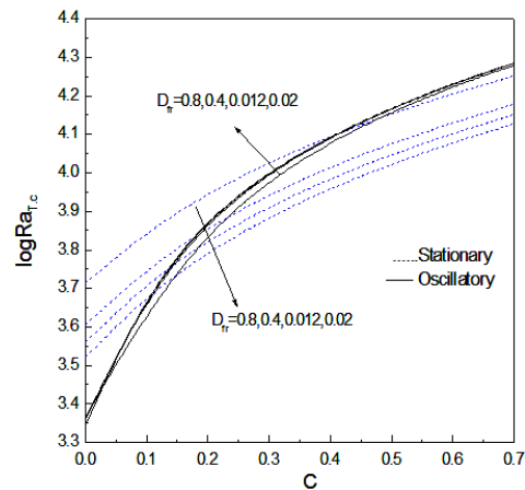
Fig. 12. Neutral stability curves for different values of D_{fr}
