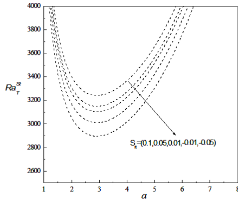
Fig. 8. Stationary neutral stability curves for different values of S_{rt}
