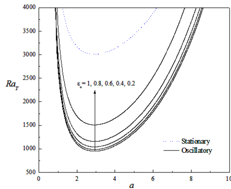
Fig. 3. Neutral stability curves for different values of \varepsilon_n
