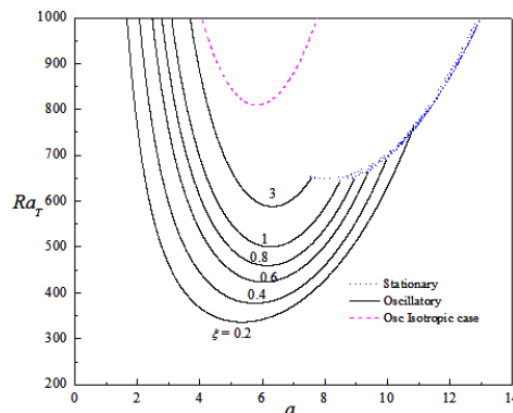
Fig. 4. Neutral stability curves for different values of \xi .
