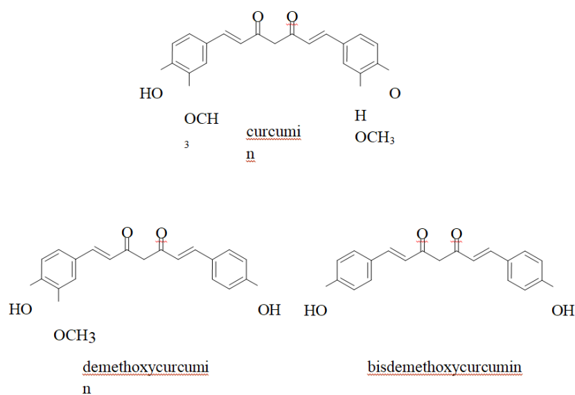
Figure 1 : Structure of the 3 major curcuminoids in turmeric
