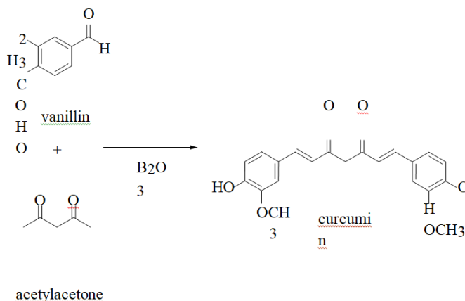
Scheme 2: Synthesis of curcumin according to Pavolini 33
