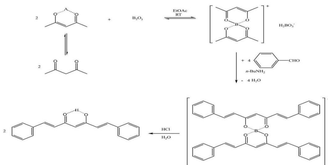
Scheme 3: Synthesis of curcuminoids according to Pabon PHARMACOLOGICAL ACTIVITY OF CURCUMIN:-
