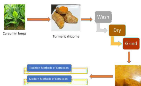
Figure 2: Steps of isolation of curcumin from turmeric
