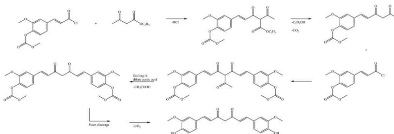
Scheme 1: Synthesis of curcumin according to Lampe
