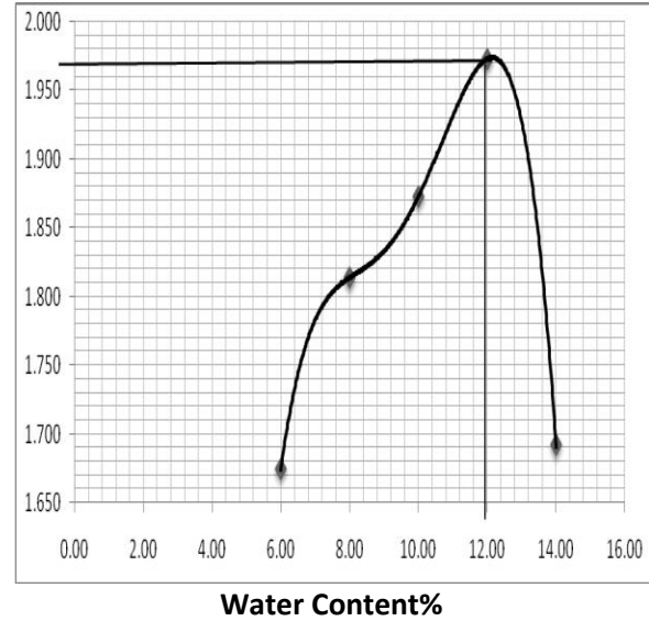
Graph 4.1.3 of Standard Proctor Result From Graph
