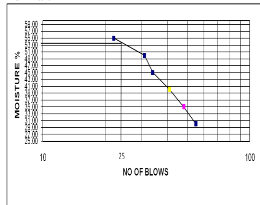
Fig 4.1.2.1: Water content Vs Number of blows.
