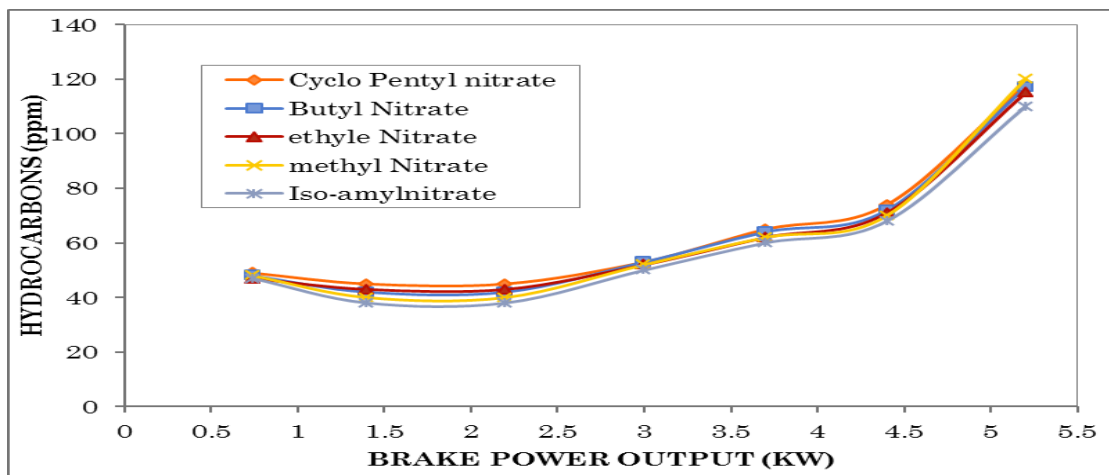
Fig. Comparison of Hydrocarbons with power output for five Fuels additives in Copper CHSI Engine.
