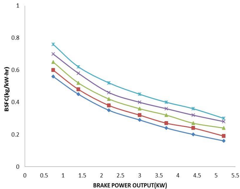
Fig. Comparison of brake specific fuel consumption with power output for five Fuels additives in Copper CHSI Engine.
