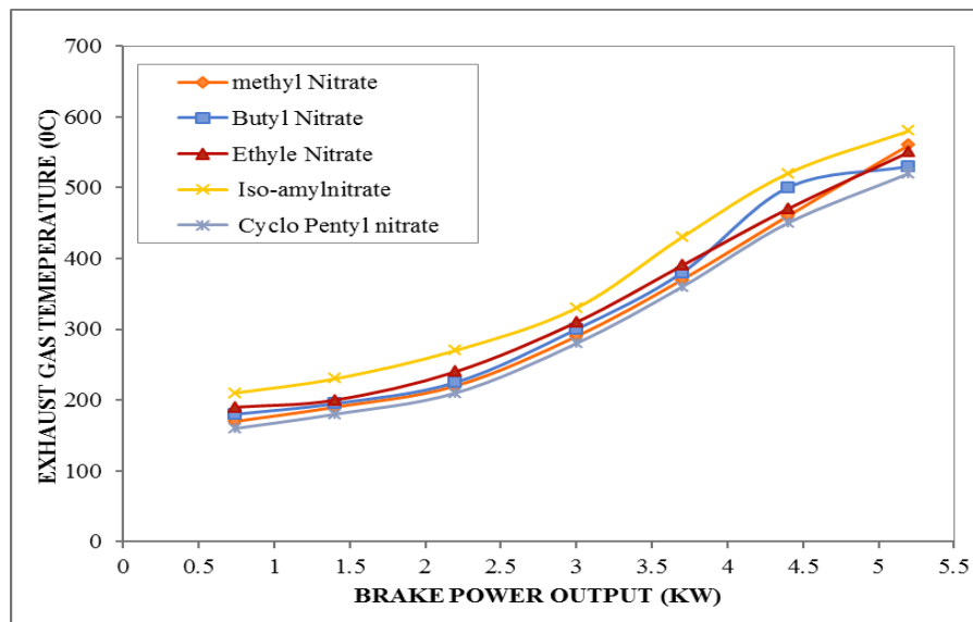
Fig Comparison of Exhaust gas temperature with power output for five Fuels additives in Copper CHSI Engine.
