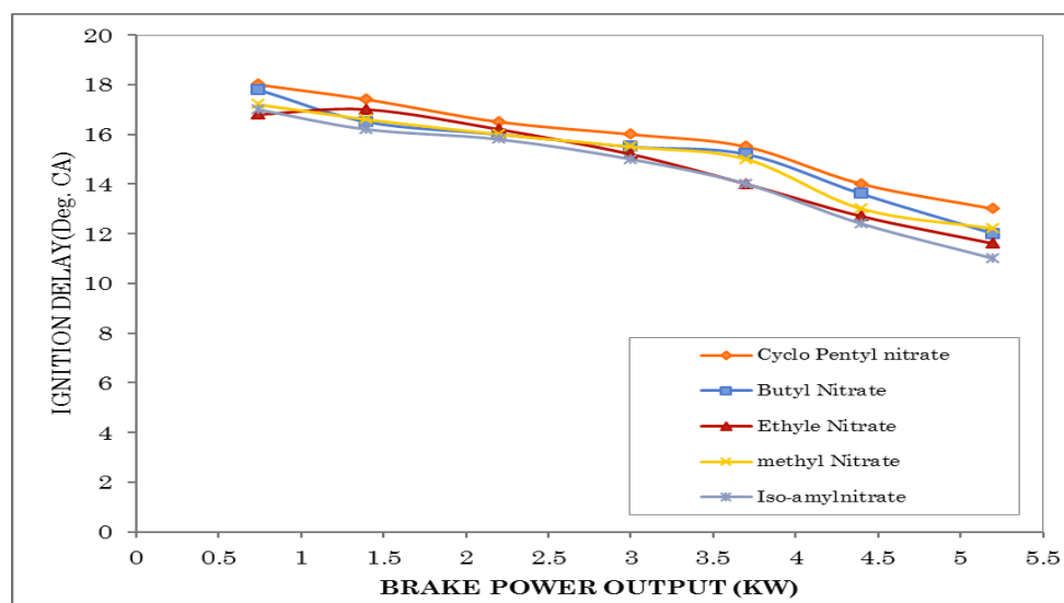
Fig. Comparison of Ignition delay with power output for five Fuels additives in Copper CHSI Engine.
