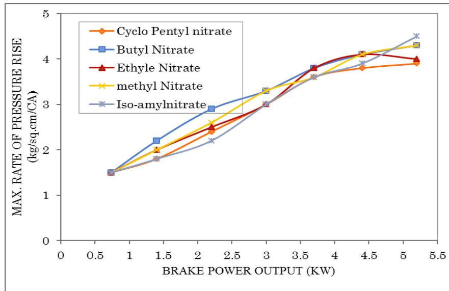
Fig. Comparison of maximum Rate of Pressure Rise with power output for five Fuels additives in Copper CHSI Engine.
