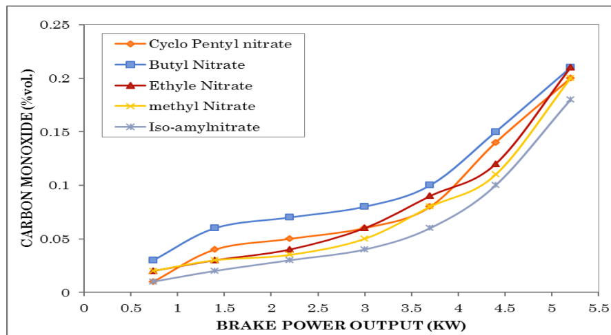
Fig. Comparison of CO emission with power output for five Fuels additives in Copper CHSI Engine.
