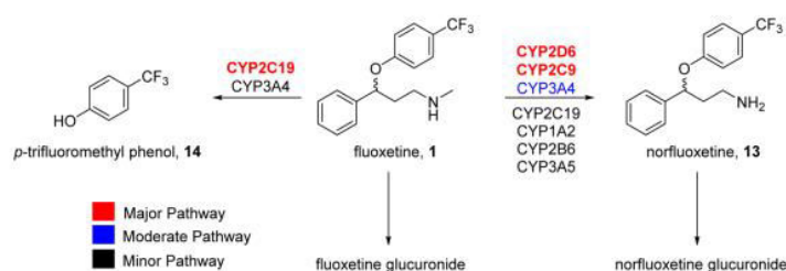
Figure 1. Structures of the oxidative and conjugative metabolites of fluoxetine 1. The major metabolite is N-desmethylfluoxetine 13, equipotent to 1, but with a significantly longer half-life. The phenolic metabolite 14 is inactive. The single enantiomers (S)-1 and (R)-1 showed divergent 2D6 metabolism.
