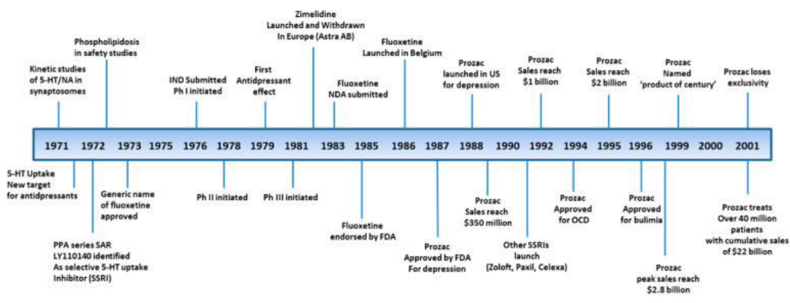
Figure 4. Timeline of the key milestones that led to the development of Prozac (1) and other SSRIs, highlighting key sales figures. Figure adapted from Wong et al. 18
