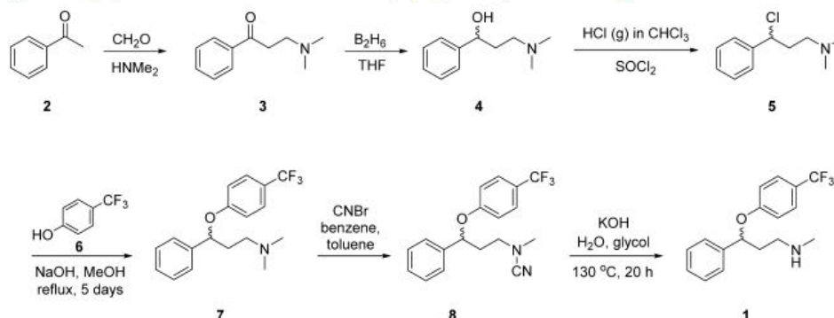
Scheme 1. Original Lilly Synthesis of Racemic Fluoxetine (1) by Molloy and Schmiegel from 1982
